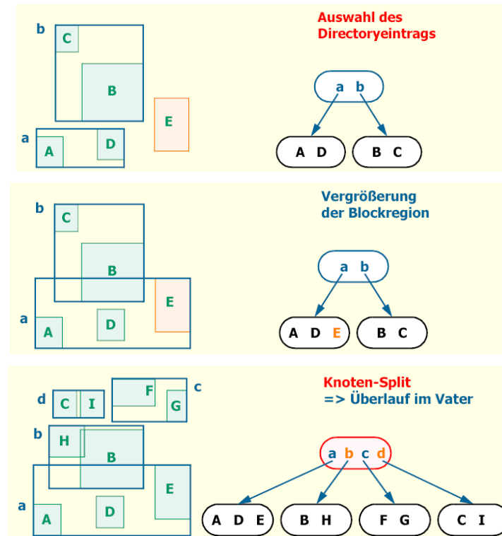
Figure 4: Animated insertion into r-trees.
